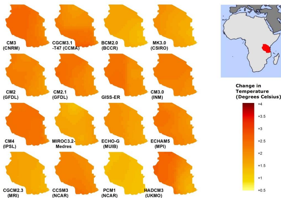
Figure 4: Comparison of climate models and change in Temperature by the 2050s under the A2 scenario
