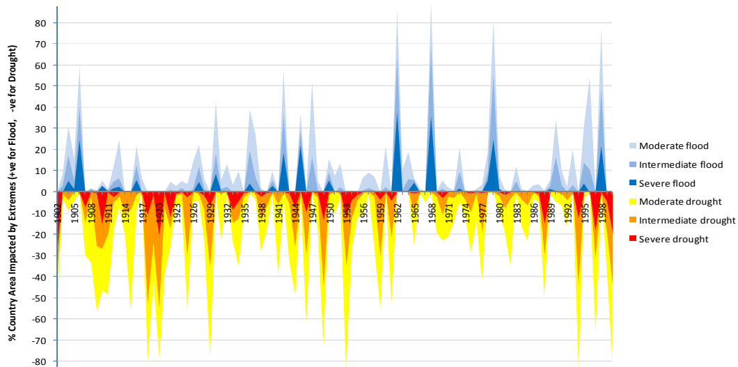
Figure 9: Extreme event frequency and impact (1900 – 2000)
