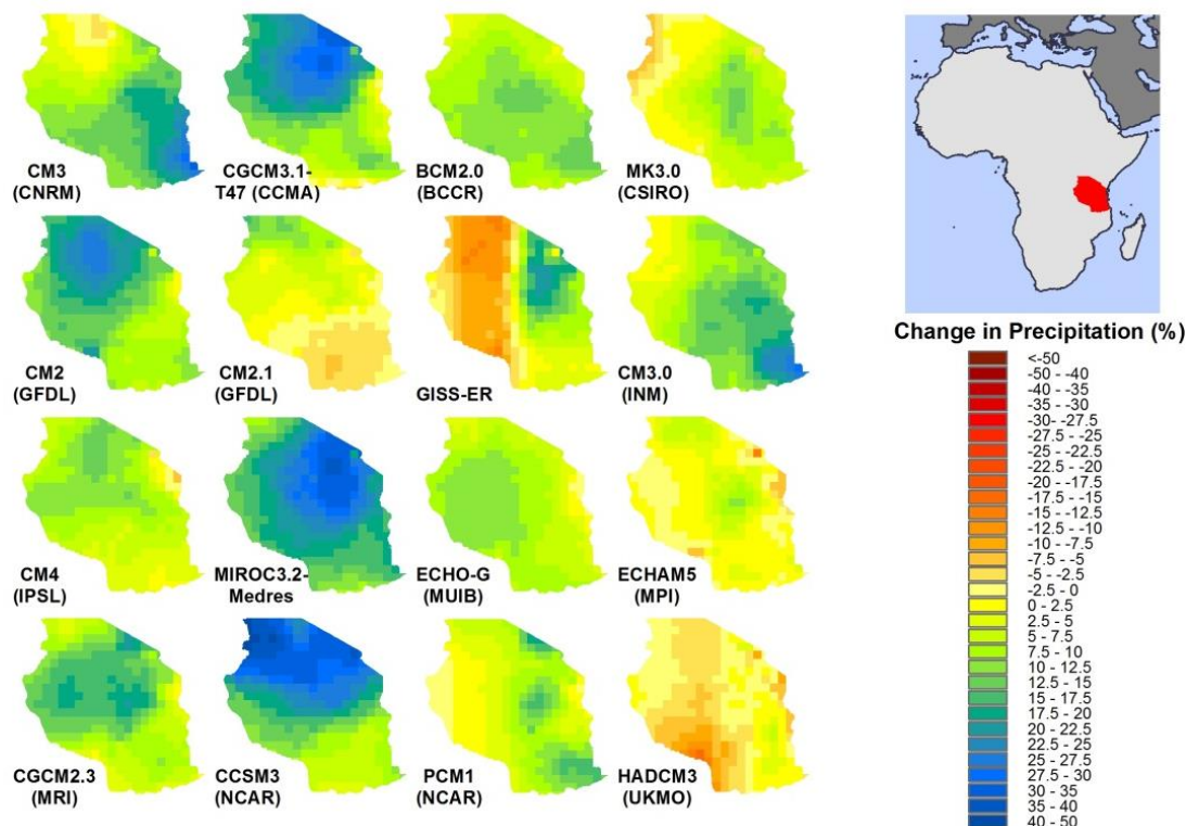
Figure 8: Comparison of climate models for percent change in annual precipitation by the 2050s under the A2 scenario
