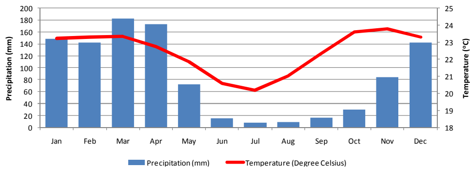
Figure 5: Average annual temperatures and precipitation in Tanzania (1901 – 2000)
