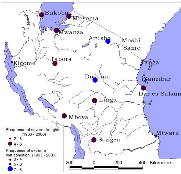
Figure 10: Frequency of droughts and floods, 1963 – 2006
